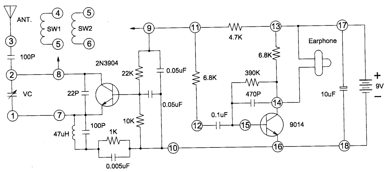
AM SW RADIO SCHEMATIC DIAGRAM
